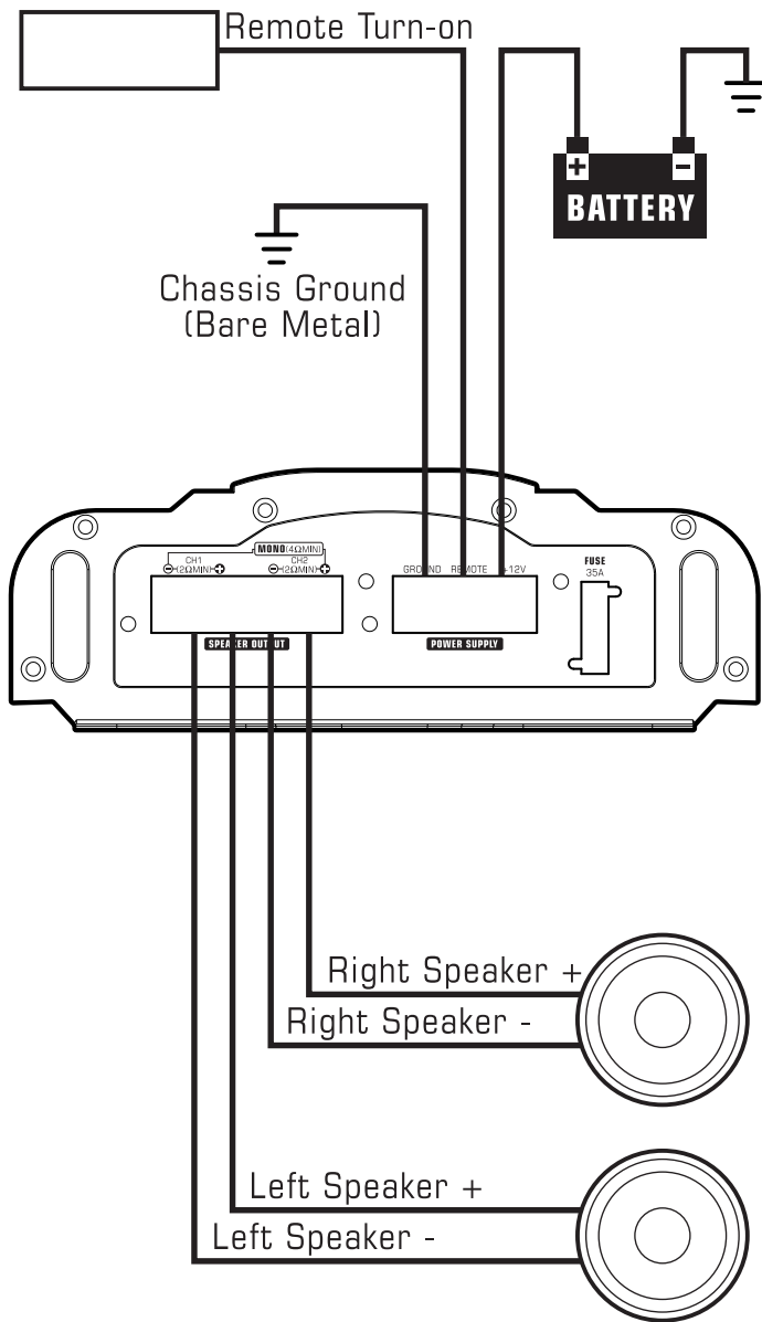
Figure 3 Connections for power and speakers
